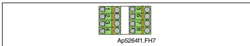
Fig. 6-11: Connector X1
