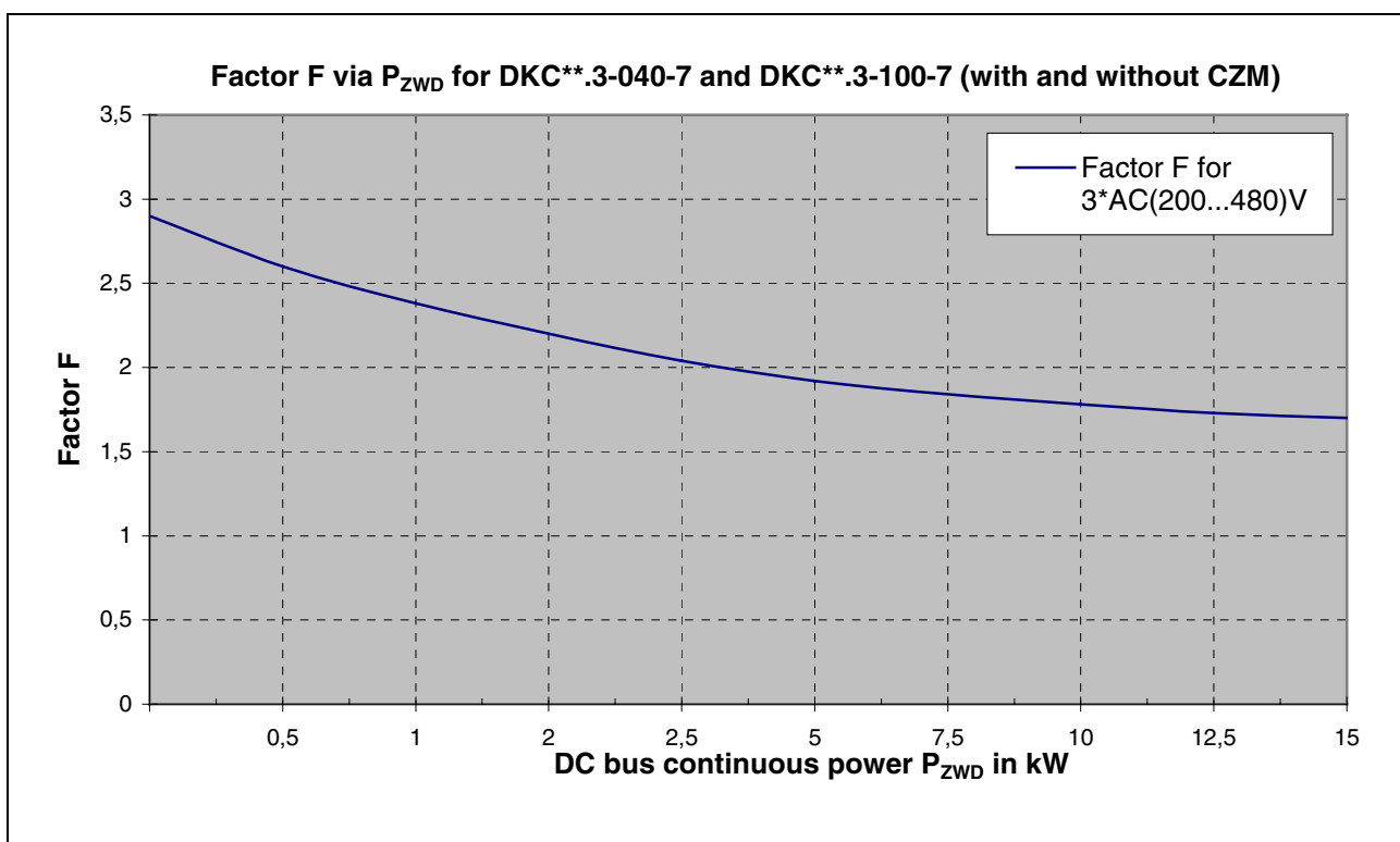
Fig. 11-9: Connected load factor for DKC**.3-040-7 and DKC**.3-100-7
