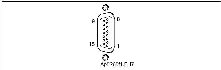
Fig. 4-81: Connector X4
