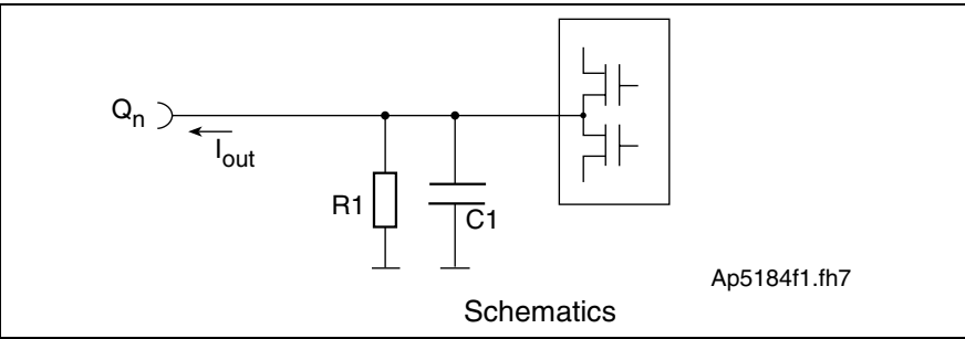
Fig. 4-69: Control outputs
