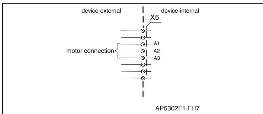
Fig. 4-94: Motor connections
