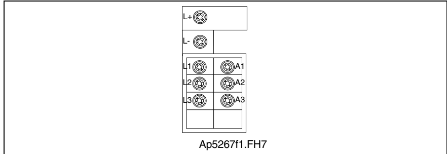
Fig. 6-35: Connector X5
