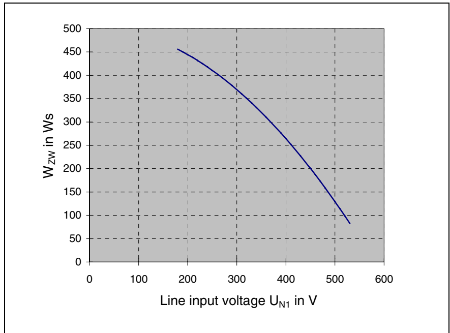
Fig. 4-19: Storable energy in the bus DKC**.3-200-7-FW
