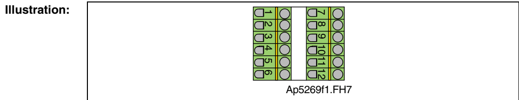
Fig. 4-122: Connector X9
