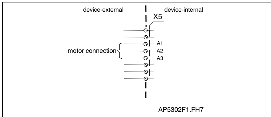
Fig. 4-94: Motor connections
