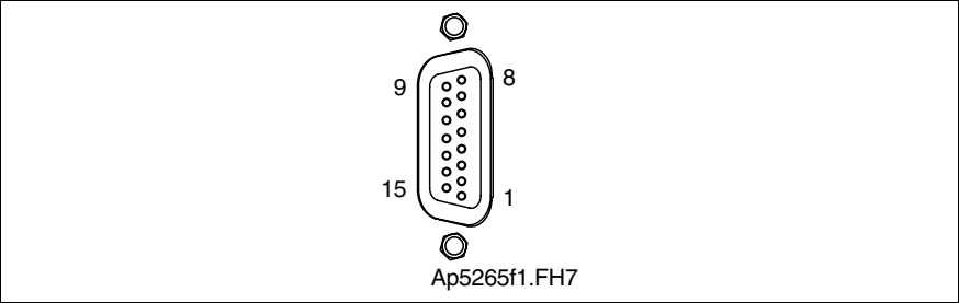
Fig. 5-30: Connector X2
