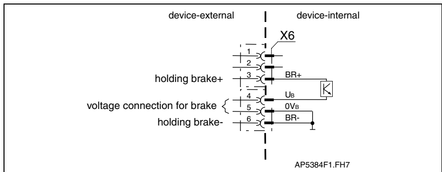
Fig. 5-64: Holding brake and voltage connection
