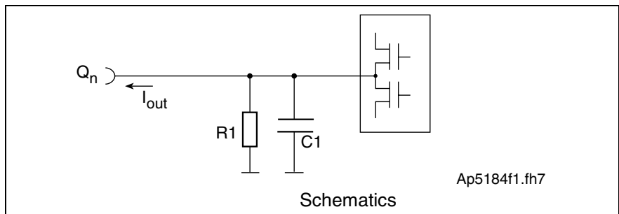
Fig. 4-69: Control outputs
