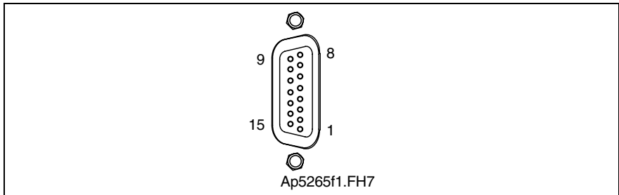
Fig. 4-57: Connector X2
