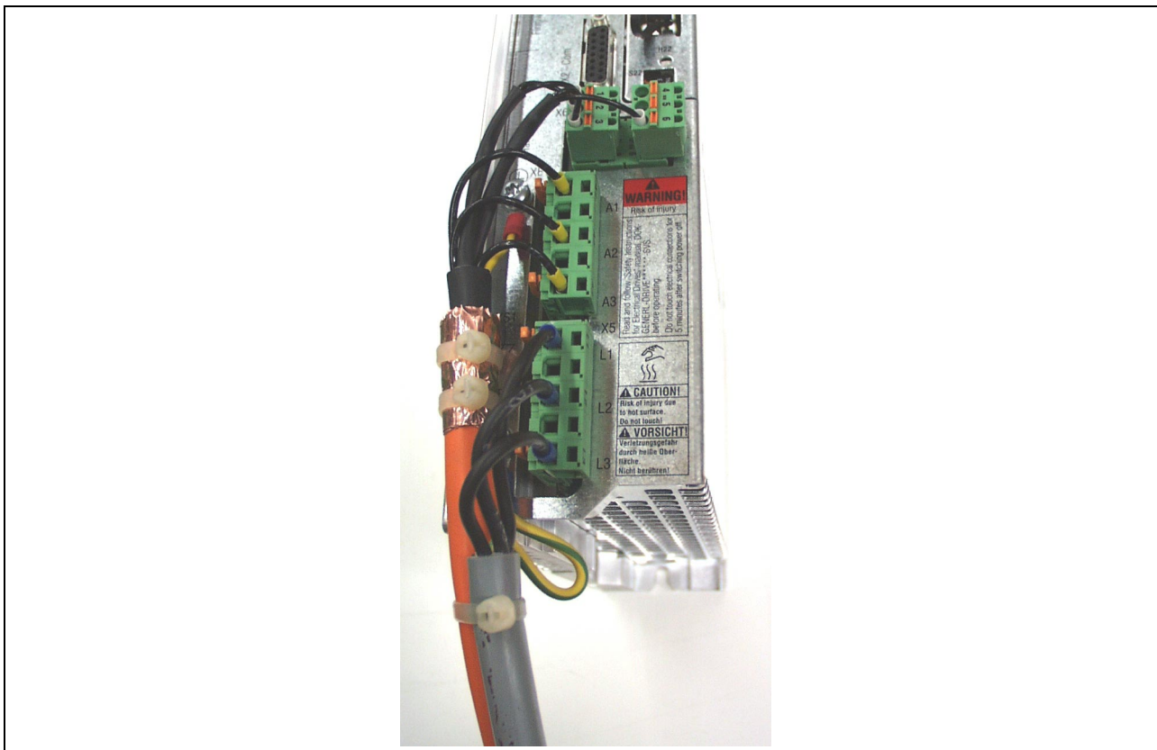
Fig. 16-27: Connection of motor and mains cable
