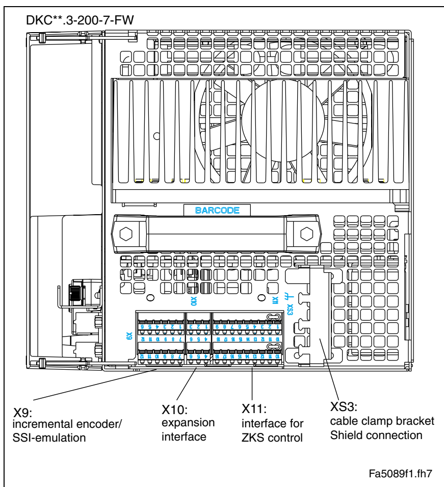
Fig. 4-46: Connections on top of unit for DKC ** .3-200-7-FW
