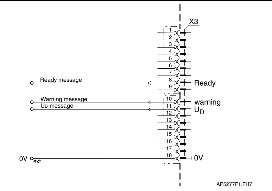
Fig. 4-69: Control outputs
