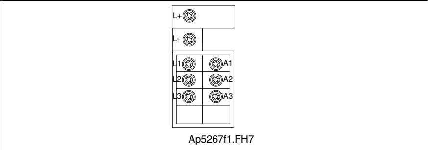
Fig. 7-8: Connector X5
