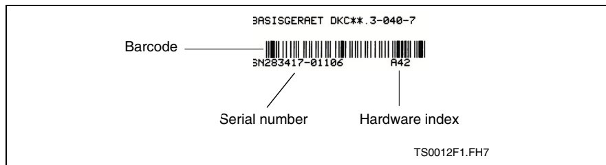
Fig. 14-2: Type plate
