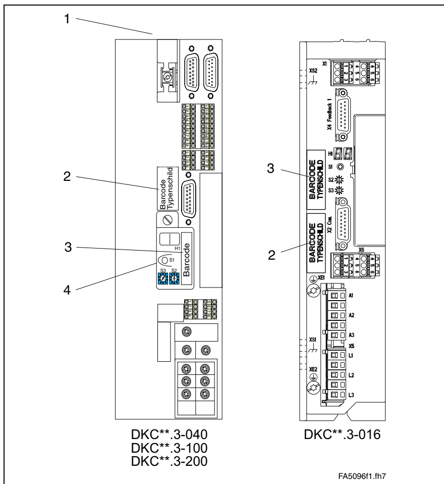
Fig. 14-1: Type plates
