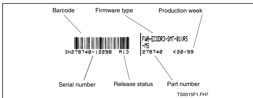
Fig. 14-4: Type plate
