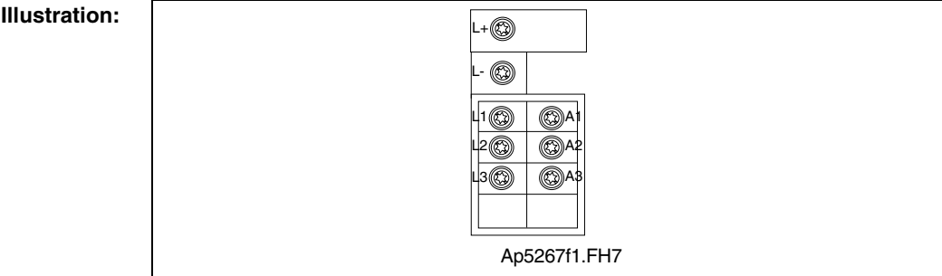
Fig. 6-35: Connector X5
