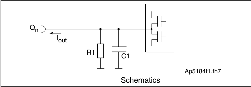
Output circuit Q 0 – Q 9:
