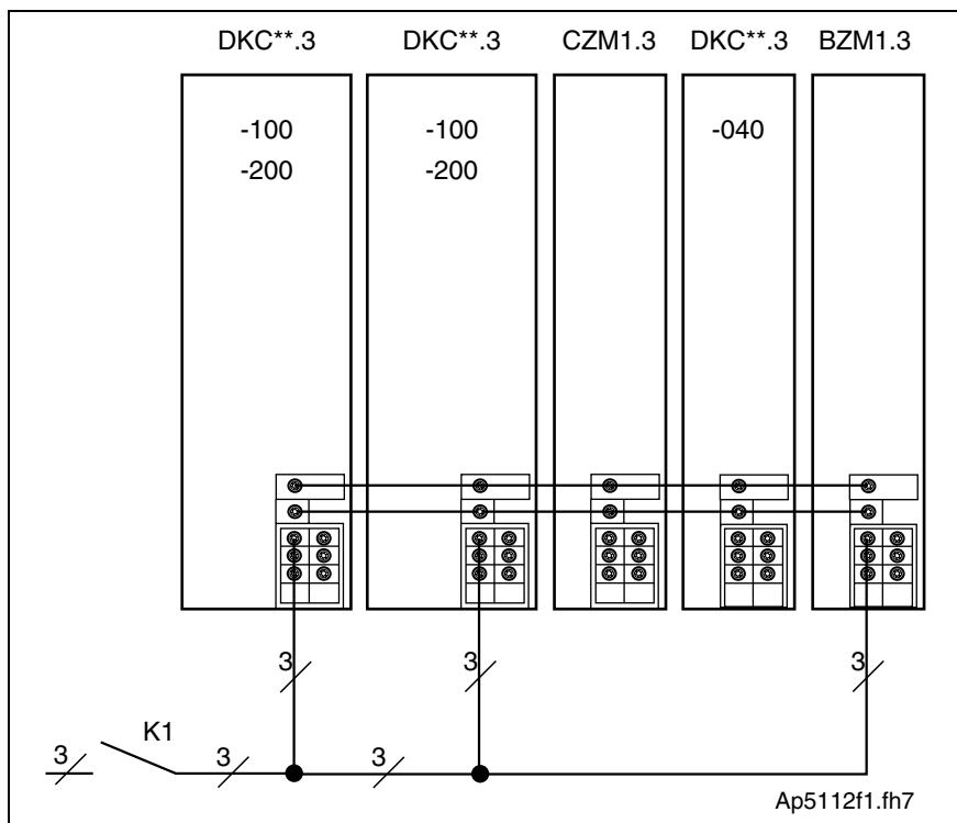
Fig. 4-25: Central supply
