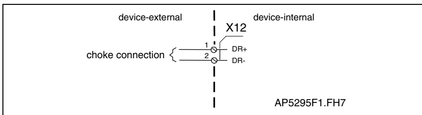
Fig. 4-154: Optional choke connection for DKC**.3-200-7
