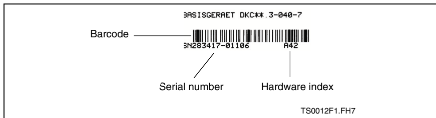
Fig. 14-2: Type plate
