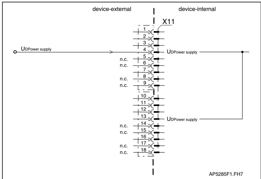
Fig. 4-147: Bb drive, Bb power supply and U D power supply
