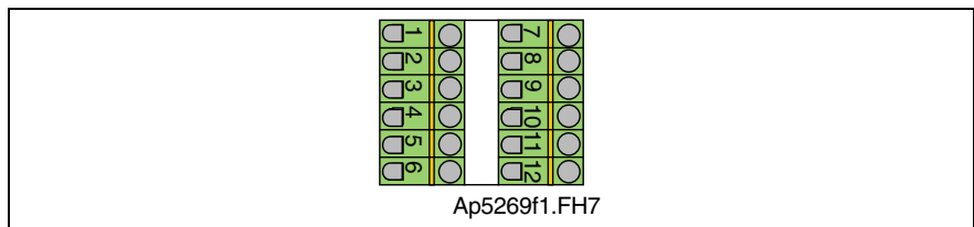
Fig. 6-17: Connector X2
