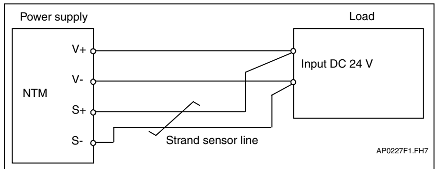
Fig. 9-6: Connecting the sensor cables NTM01.1-024-004 and NTM01.1-024-006
