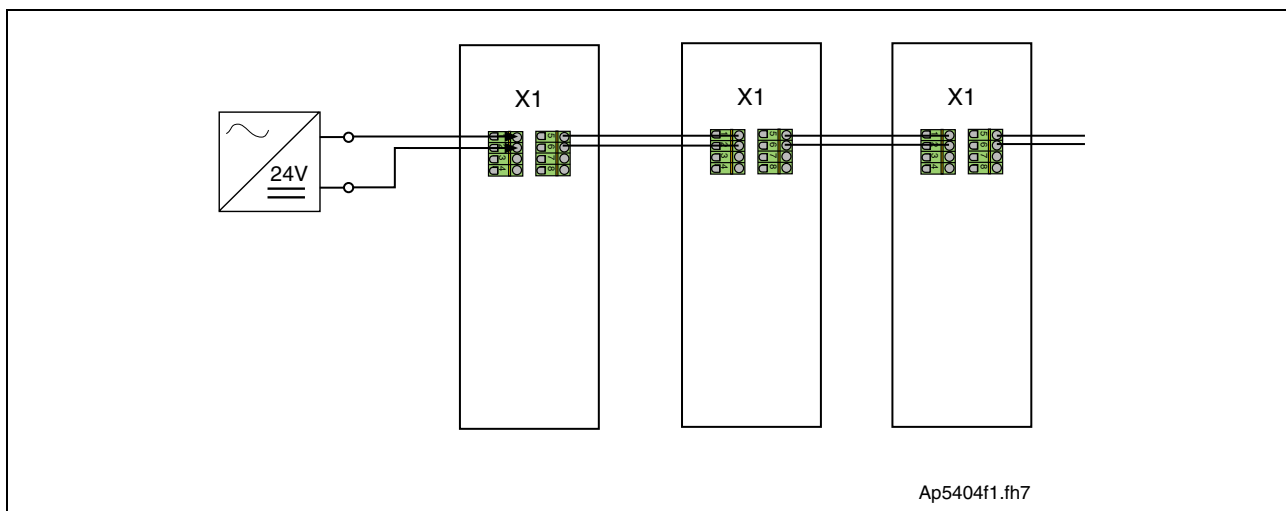
Fig. 16-11: Looping through the control voltage
