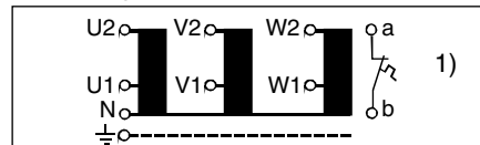
Block diagram
