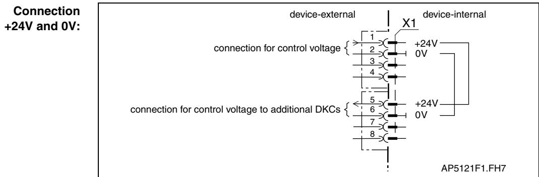
Fig. 4-51: Connections for control voltage
